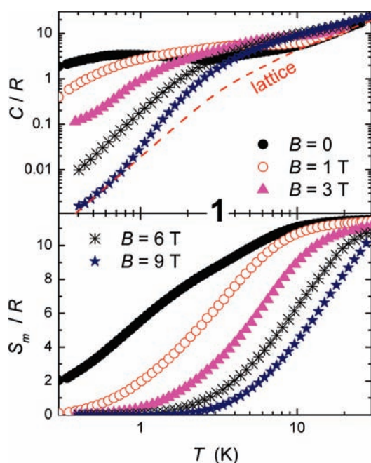
Figure 6. Top: temperature dependencies of the heat capacity of 1 normalized to the gas constant R collected for B = 0, 1, 3, 6, and 9 T. Dashed line is the fitted lattice contribution. Bottom: temperature dependencies of the experimental magnetic entropy for several B , as obtained from the respective magnetic contributions to the total heat capacity.
