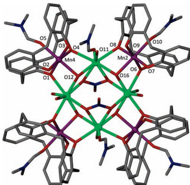
Figure 2. Molecular structure of 1 , showing the coordination environments around the \text{Mn}^{\text{III}} and \text{Gd}^{\text{III}} centers. Hydrogen atoms, hydroxide anions, and cocrystallized DMF molecules are omitted for clarity. Color code as in Figure 1; Ln, green.
